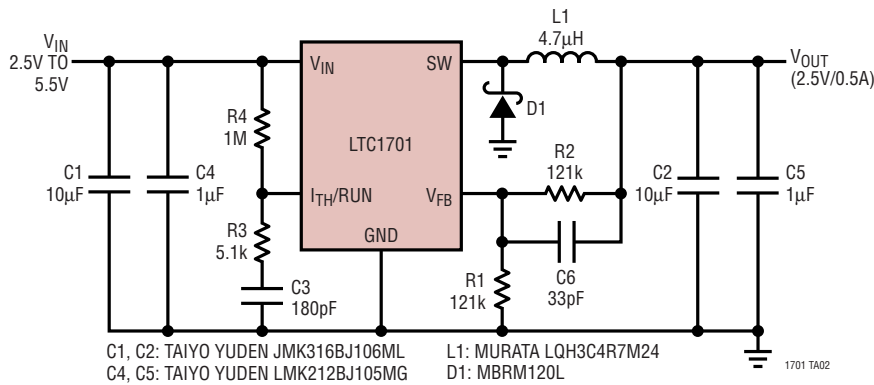
All Ceramic Capacitor 2.5V Converter
