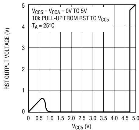
Figure 5. \overline{\text{RST}} Output Voltage Characteristics of the Circuit in Figure 4
