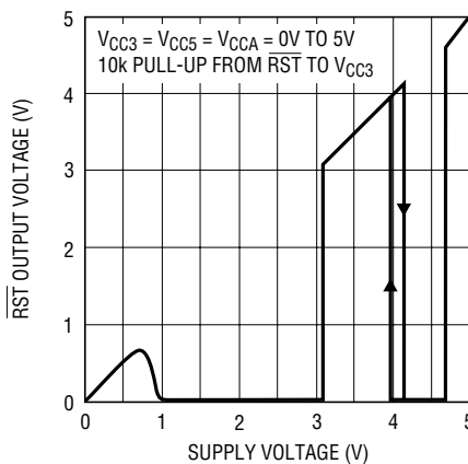
Figure 3. \overline{RST} Voltage vs Supply Voltage
