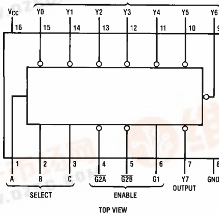
Pin Assignments for DIP, SOIC, SOP and TSSOP DATA OUTPUTS
