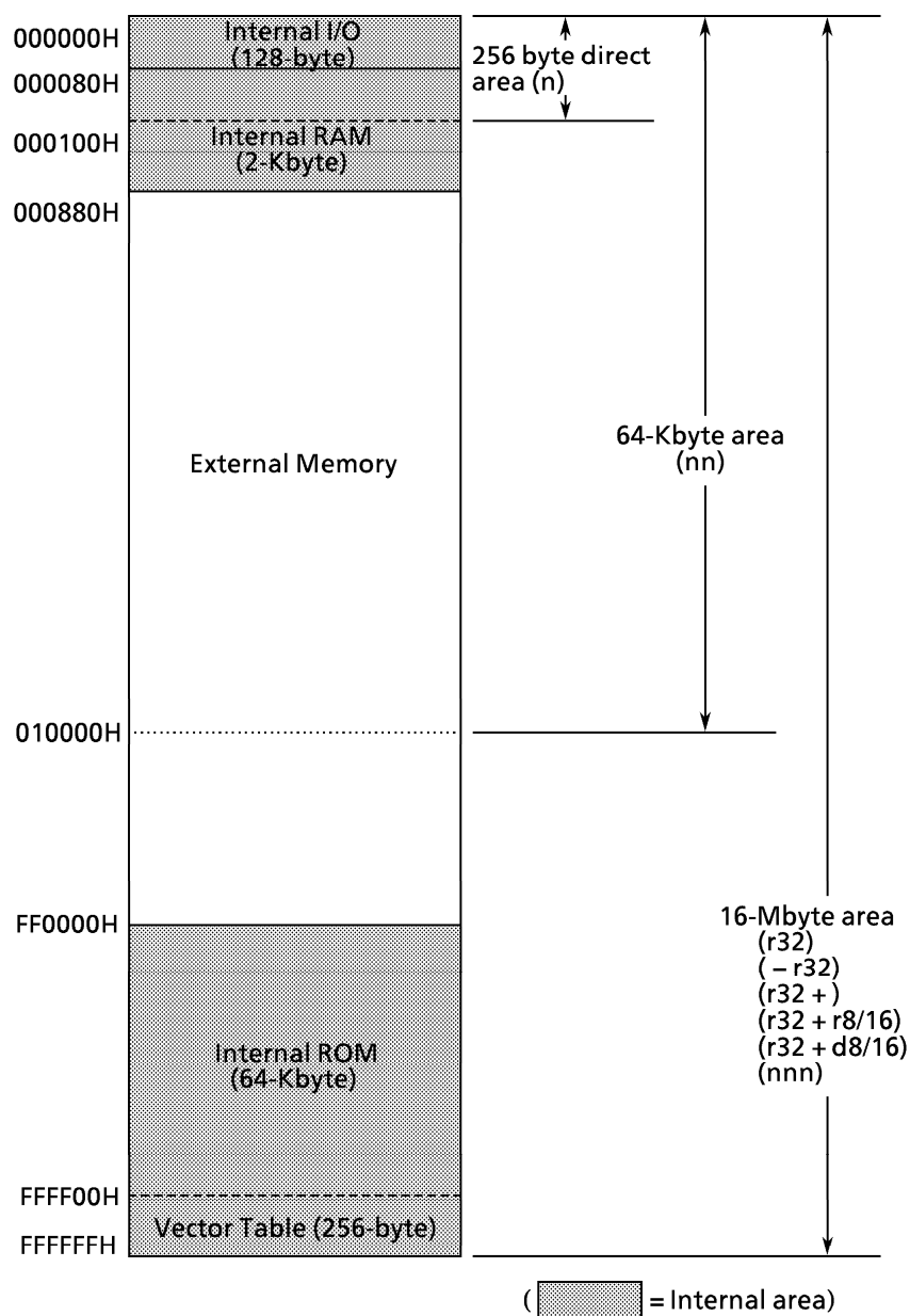
Figure 3.2.1 Memory map
