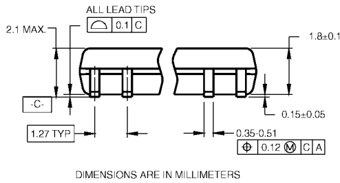
DIMENSIONS ARE IN MILLIMETERS
