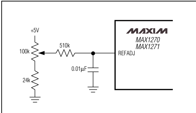
Figure 1. Reference-Adjust Circuit
