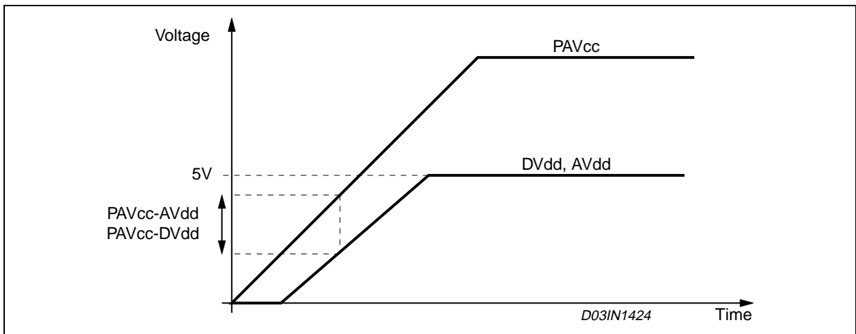
Figure 21. Power-UP Sequence
