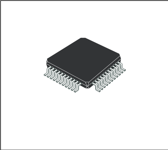
TQFP44 (10x10x1.40mm) with Slug Down
