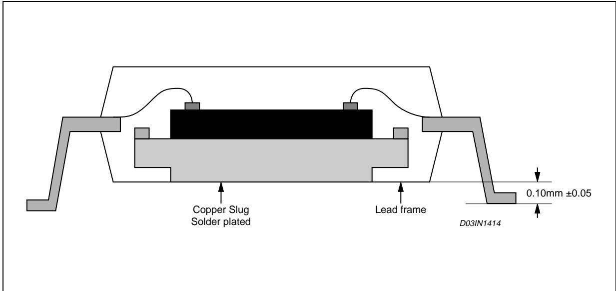
Figure 24. Soldering Information
