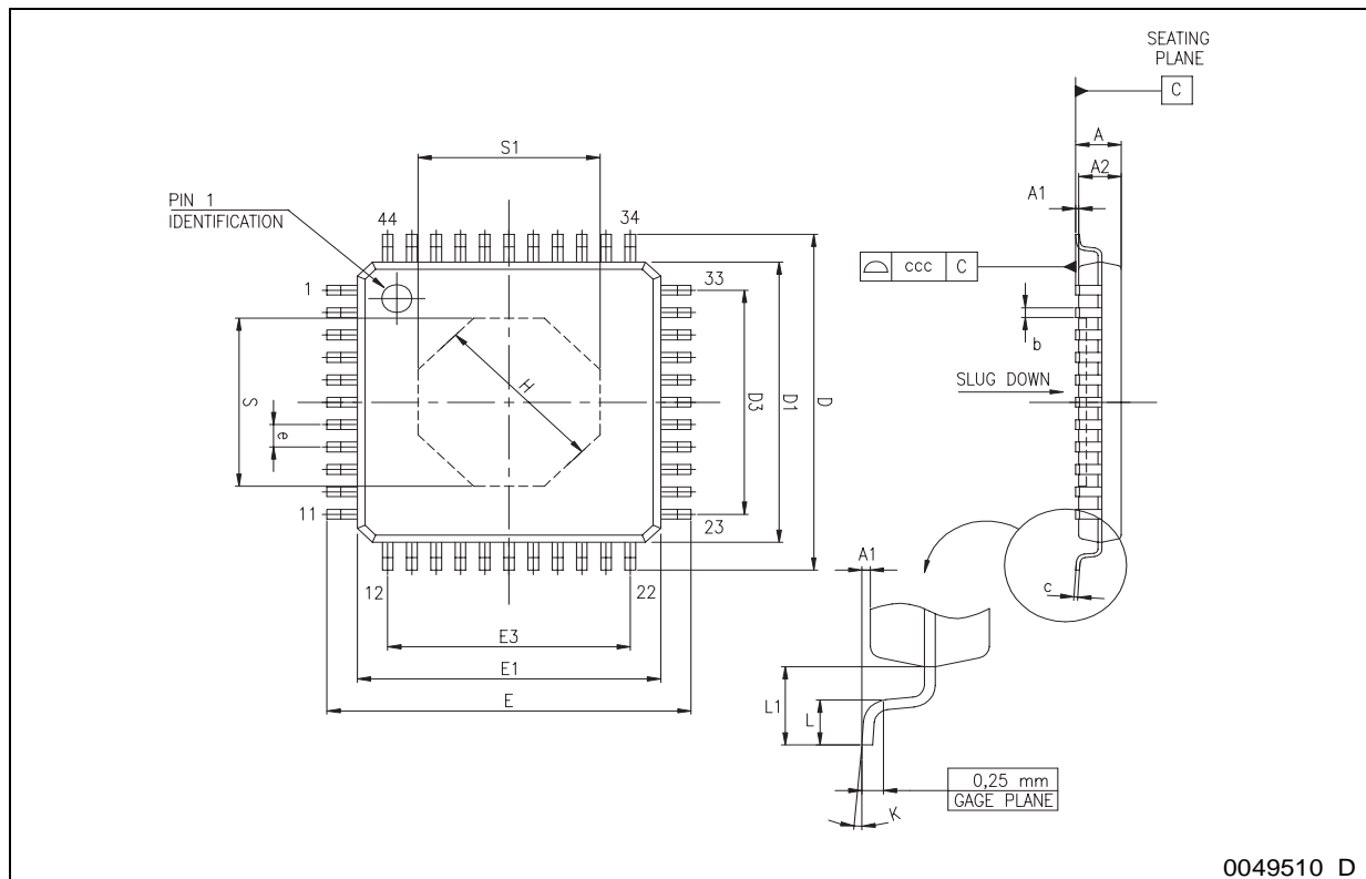
TQFP44 (10x10x1.40mm) with Slug Down
