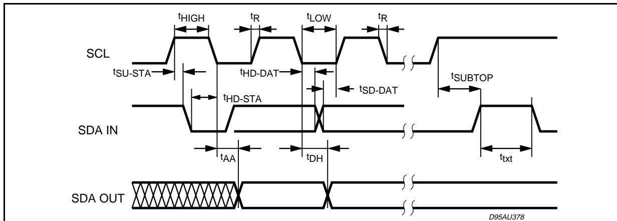
Figure 5. I 2 C Bus timing diagram
