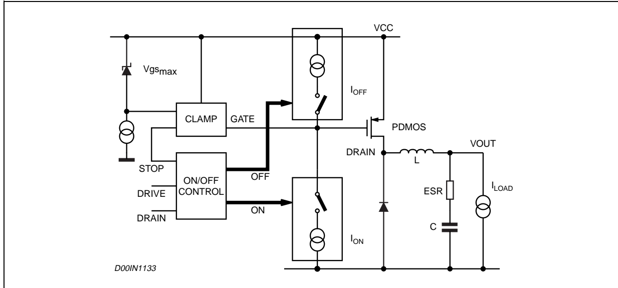
Figure 5. Driving Circuitry
