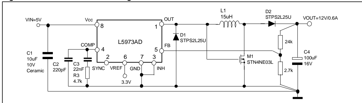
Figure 12. Buck-Boost regulator
