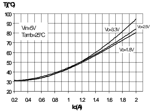
Figure 8. Junction Temperature vs Output Current
