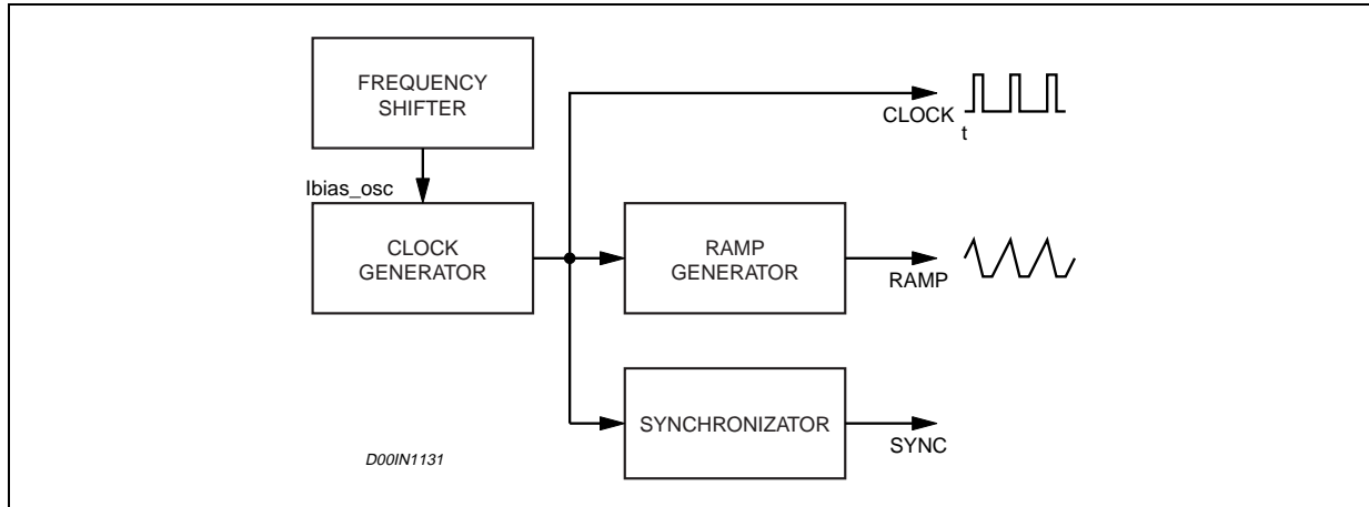
Figure 3. Oscillator Circuit
