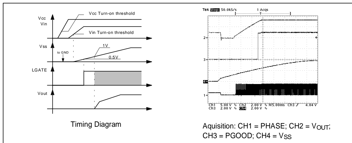
Figure 2. Soft Start
