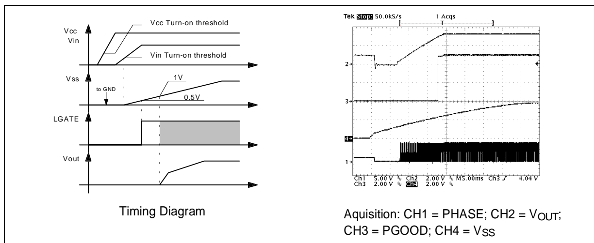
Figure 2. Soft Start
