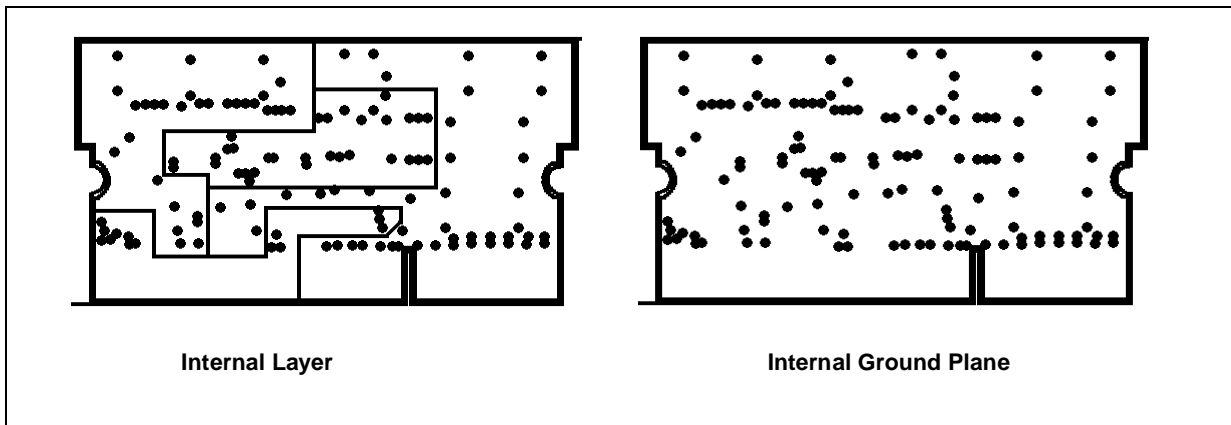
Figure 14. PCB and Components Layouts
