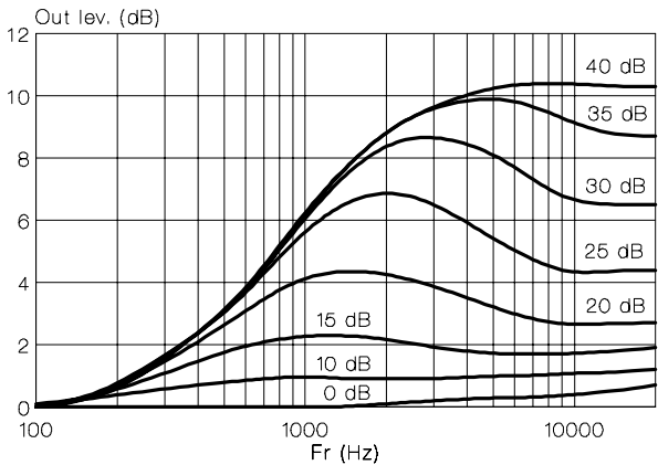
Figure 49: Dolby-B Table
