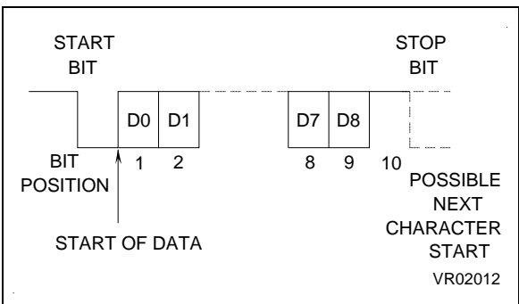
Figure 37. Character Format
