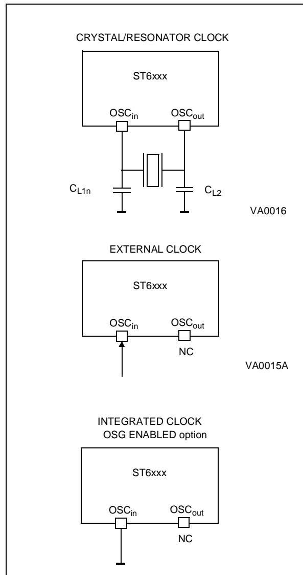
Figure 9. Oscillator Configurations
