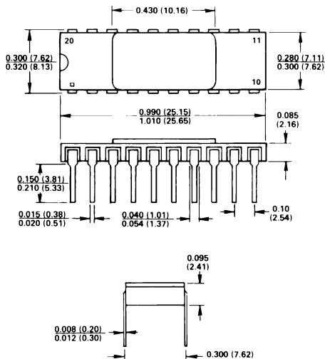
20-Pin Ceramic DIP (D-20)
