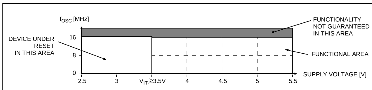
Figure 62. Low LVD Threshold Versus V_{DD} and f_{OSC} for ROM devices 2)3)
