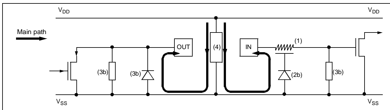
Figure 87. Multisupply Configuration
