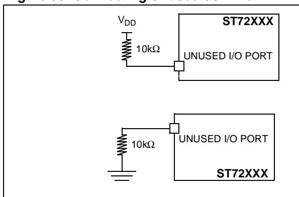
Figure 80. Connecting Unused I/O Pins
