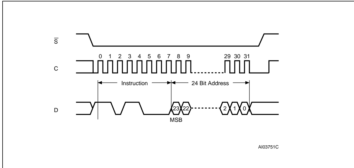
Figure 14. Sector Erase (SE) Sequence
