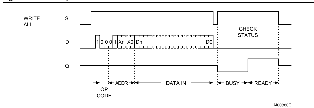
Figure 7. WRAL Sequence
