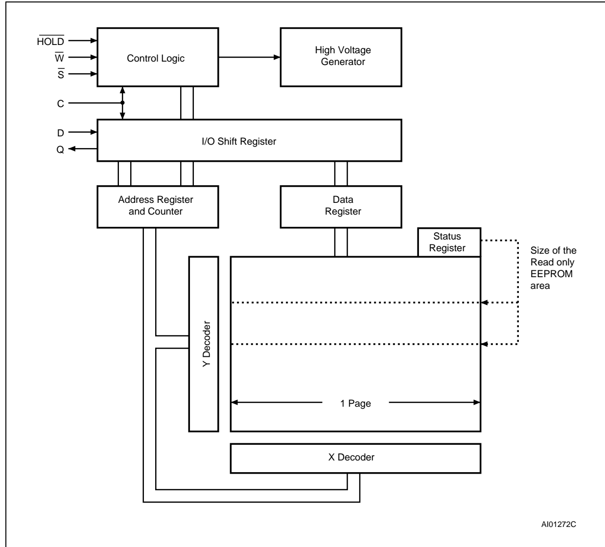
Figure 8. Block Diagram
