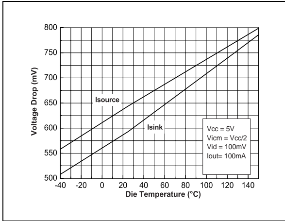
Voltage Drop vs Temperature (Iout=100mA)
