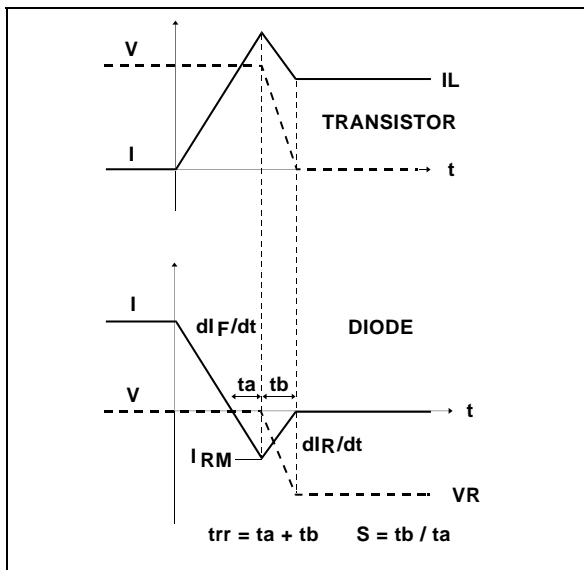
Fig. C: TURN-ON CHARACTERISTICS
