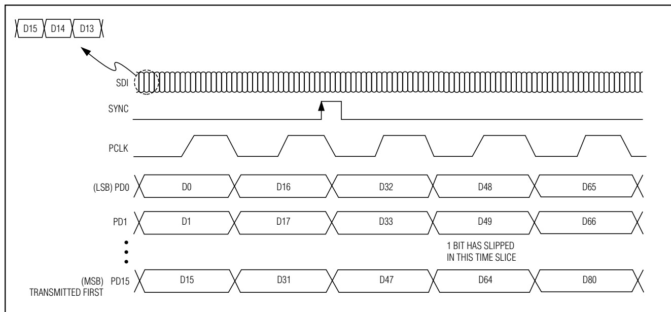
Figure 4. Timing Diagram
