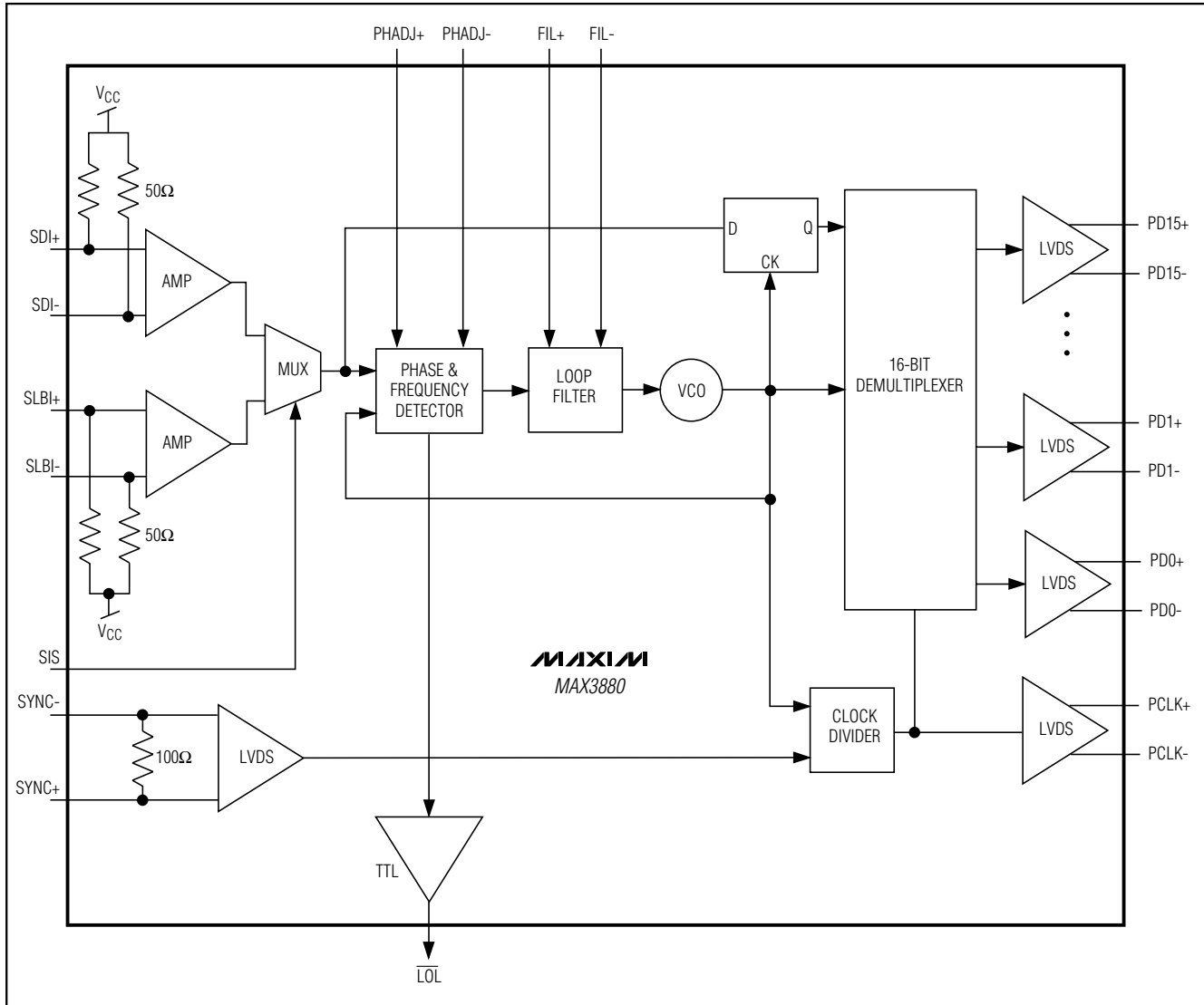
Figure 3. MAX3880 Functional Diagram
