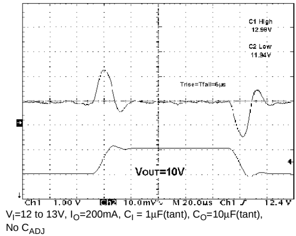
Figure 23 : Line Transient
