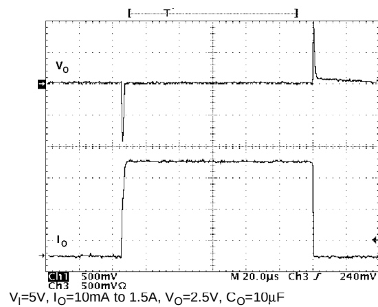
Figure 16 : Load Transient
