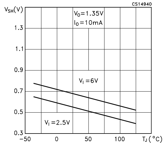
Figure 5 : Shutdown Voltage vs Temperature
