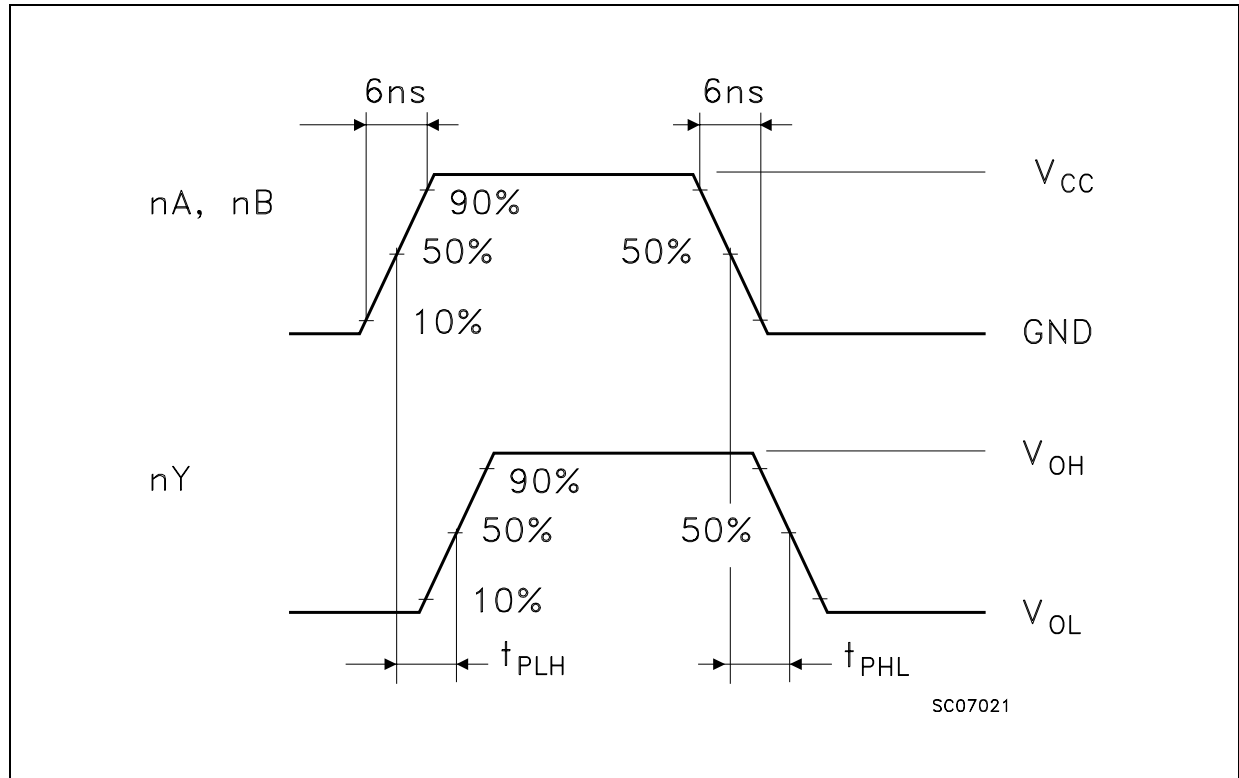
WAVEFORM 1: PROPAGATION DELAY TIME ( f=1\text{MHz} ; 50% duty cycle)
