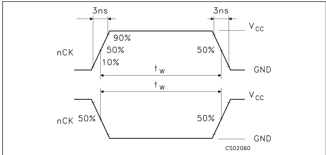
WAVEFORM 3 : CLOCK PULSE WIDTHS (f=1MHz; 50% duty cycle)
