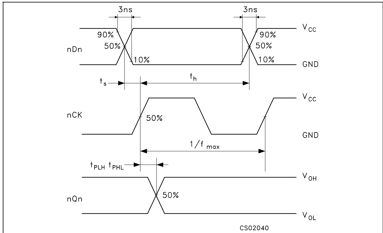
WAVEFORM 1 PROPAGATION DELAYS, SETUP AND HOLD TIMES, MAXIMUM CLOCK FREQUENCY ( f=1\text{MHz} ; 50% duty cycle)
