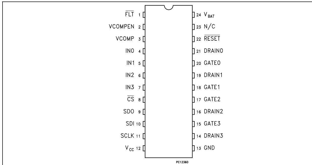
Figure 2 : Pin Configuration
