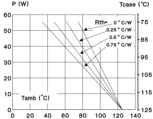
Fig. 2: Correlation between maximum RMS power dissipation and maximum allowable temperatures (Tamb and Tcase) for different thermal resistances (Rth) for heatsink + contact.
