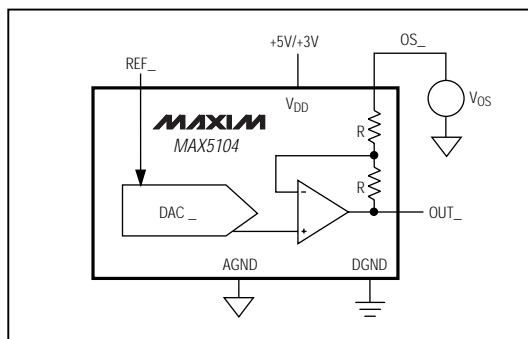
Figure 10. Setting \text{OS}_- for Output Offset
