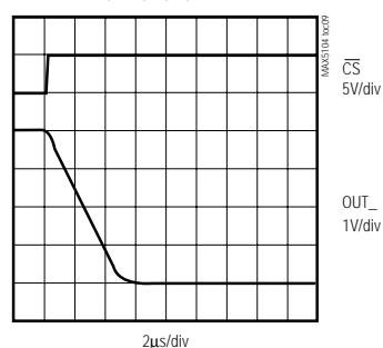
DYNAMIC RESPONSE FALL TIME
