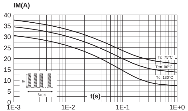
Fig. 5-2: Non repetitive surge peak forward current versus overload duration. (Maximum values, per diode) (ISOWATT220AB).
