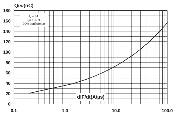
Fig. 6-2: Reverse recovery charges versus dI_F/dt (modulation diode).
