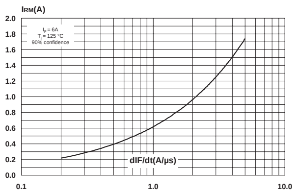
Fig. 7-1: Peak reverse recovery current versus dI_F/dt (damper diode).
