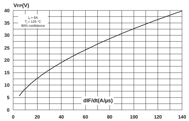
Fig. 9-1: Forward recovery time versus dI_F/dt (damper diode).
