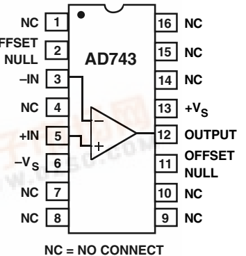
16-Lead SOIC (R) Package
