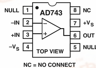
8-Lead Plastic Mini-DIP (N)
