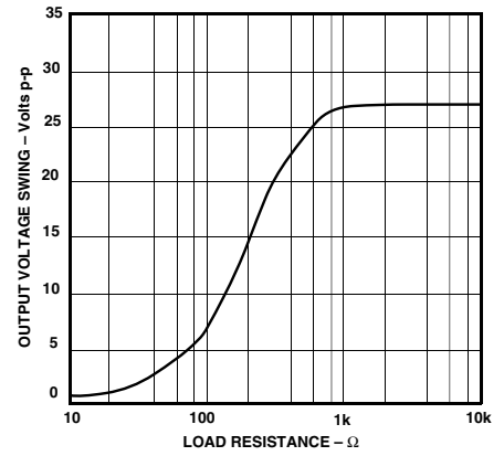
TPC 3. Output Voltage Swing vs. Load Resistance
