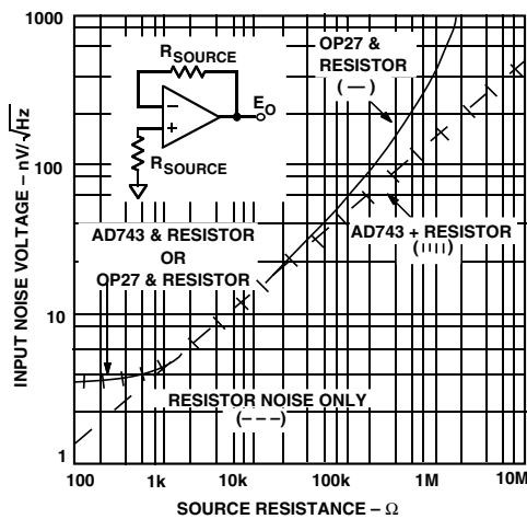
Figure 1. Total Input Noise Spectral Density @ 1 kHz vs. Source Resistance
