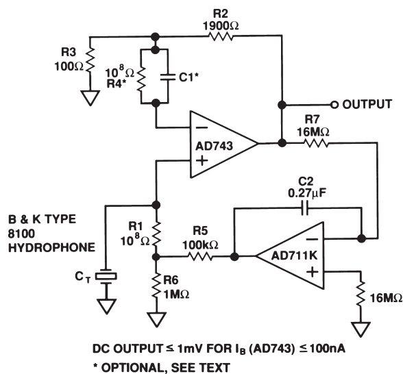
Figure 14c. A Hydrophone Amplifier Incorporating a DC Servo Loop
