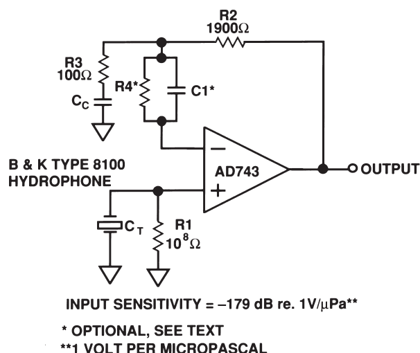
Figure 14b. An AC-Coupled, Low Noise Hydrophone Amplifier
