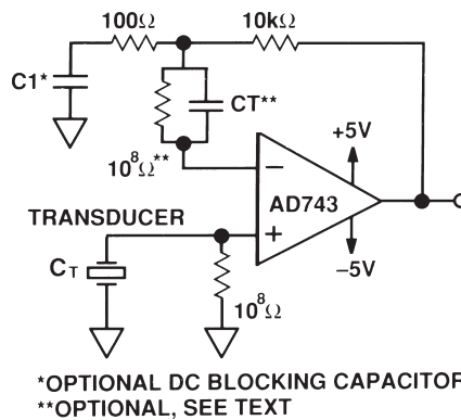
Figure 11. A Piezoelectric Transducer
