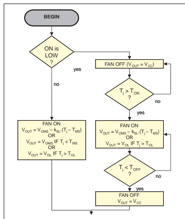
Fig. 6: FSCT behavior flow-chart.
