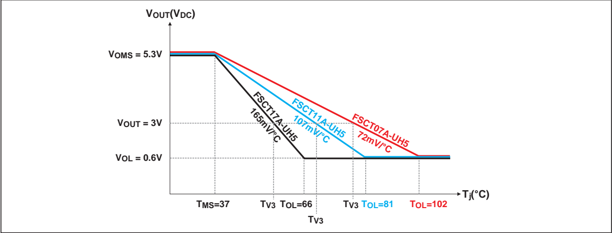
Fig. 3: Temperature slopes.
