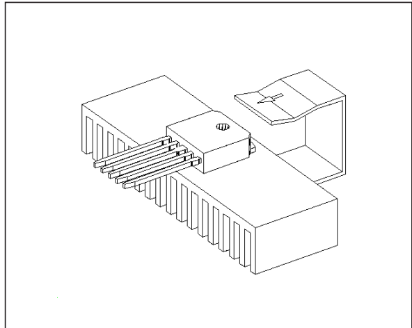
Fig. 10: IPPAK mounted with a U-clip.
