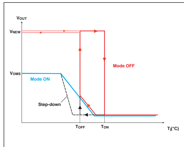
Fig. 12: Modified characteristics.
