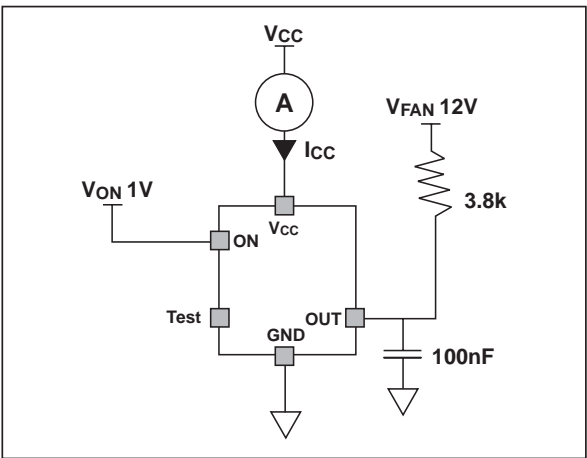
Fig. 5: I_{CC} versus V_{CC} test circuit (mode ON).
