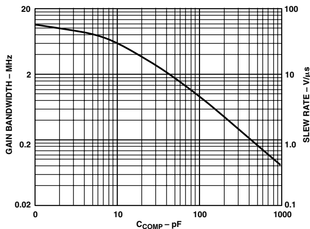
Figure 29. Gain Bandwidth and Slew Rate vs. C_{COMP}
