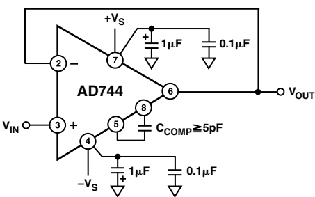
Figure 30. AD744 Connected as a Unity Gain Voltage Follower
