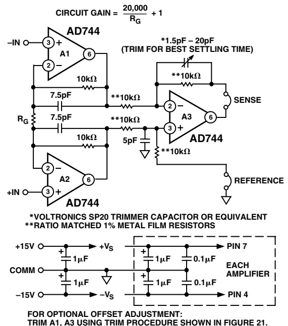
Figure 36. A High Performance, 3 Op Amp Instrumentation Amplifier Circuit
