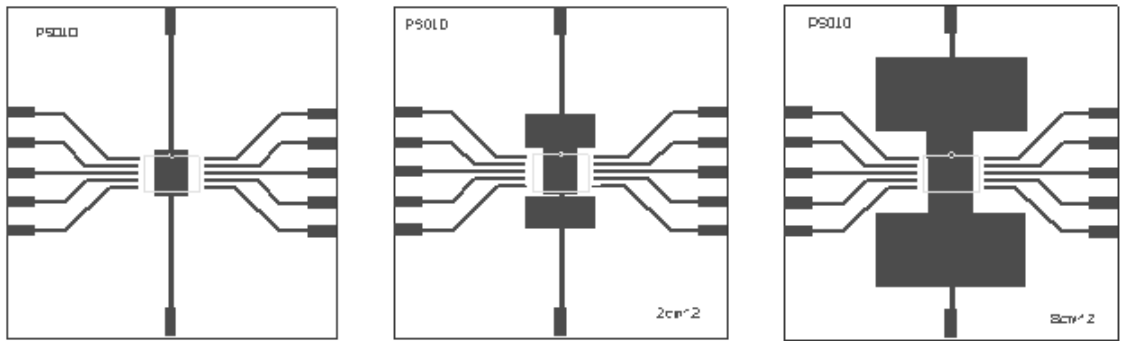
Layout condition of R_{th} and Z_{th} measurements (PCB FR4 area= 58mm x 58mm, PCB thickness=2mm, Cu thickness=35 \mu m, Copper areas: from minimum pad lay-out to 8cm 2 ).
