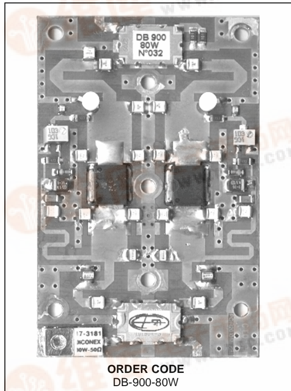
MECH. SPECIFICATION L=80 mm W=50 mm H=10 mm
