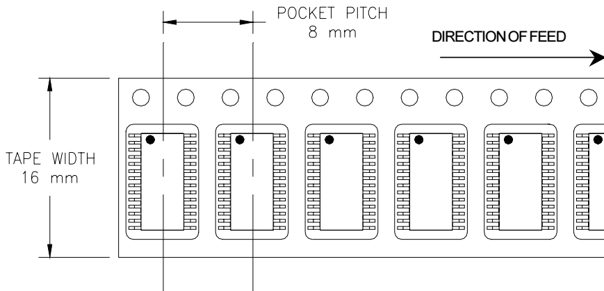
Figure 17: Tape Dimensions
