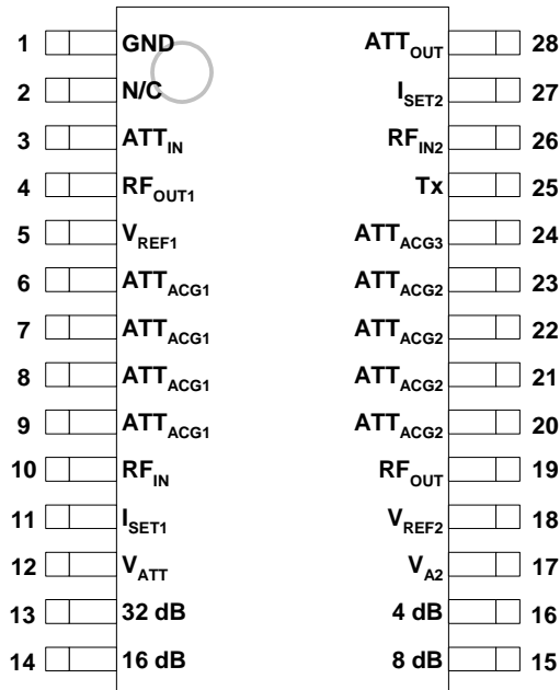
Figure 3: Pin Out
