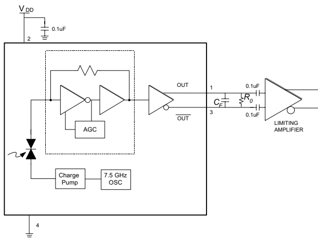
Figure 14: Application Schematic
