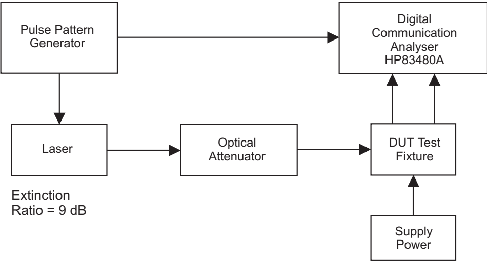
Figure 11: Test Setup for Eye Measurements
