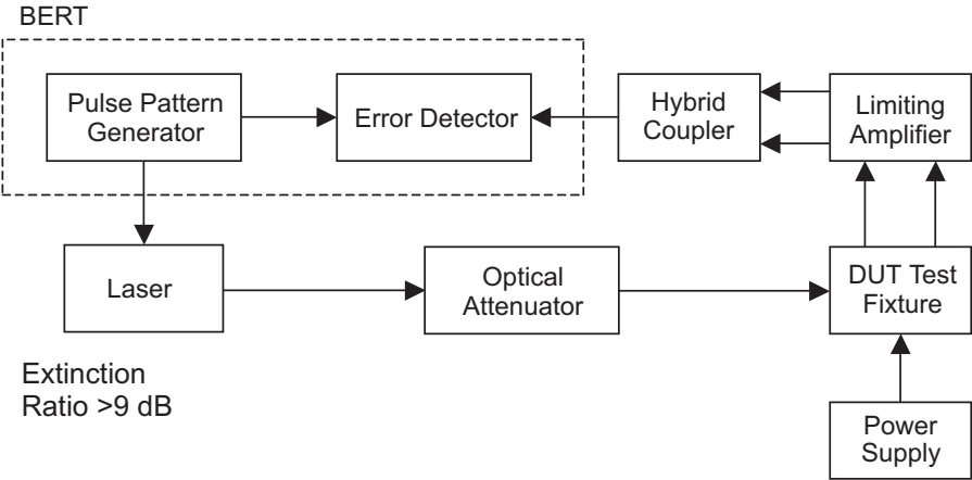
Figure 10: Test Setup for Sensitivity Measurements
