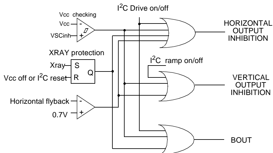
Figure 15. Safety Functions Block Diagram
