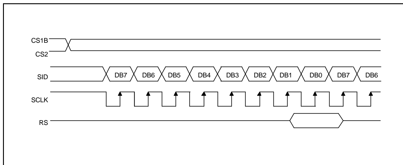
Figure 3. 4 Pin SPI serial Interface Timing (RS used)
