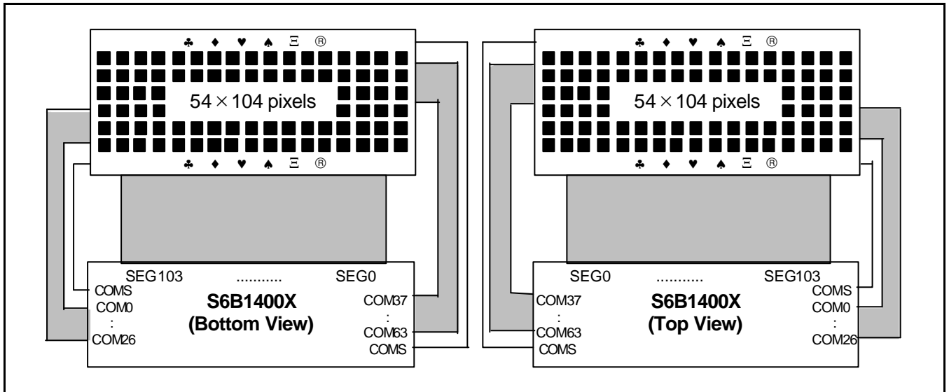
Figure 37. SHL = 1, ADC = 1
