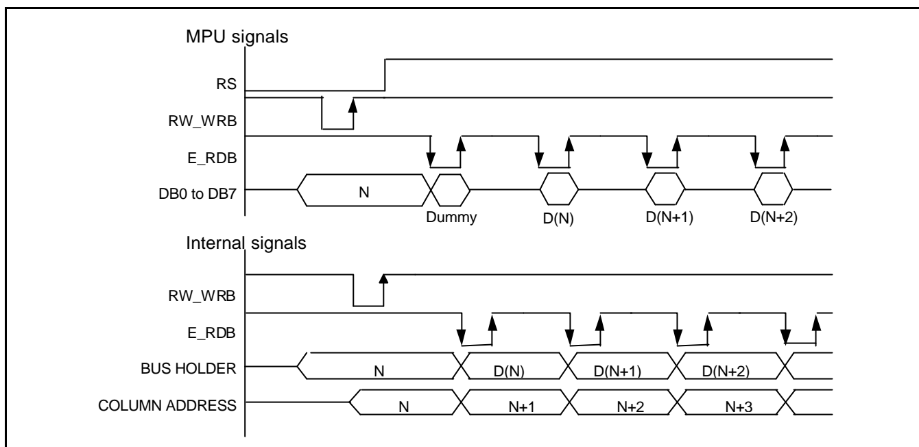
Figure 6. Read Timing
