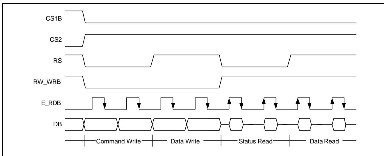
Figure 2-1. 6800-Series MPU Interface protocol (PS="H", C68="H")
