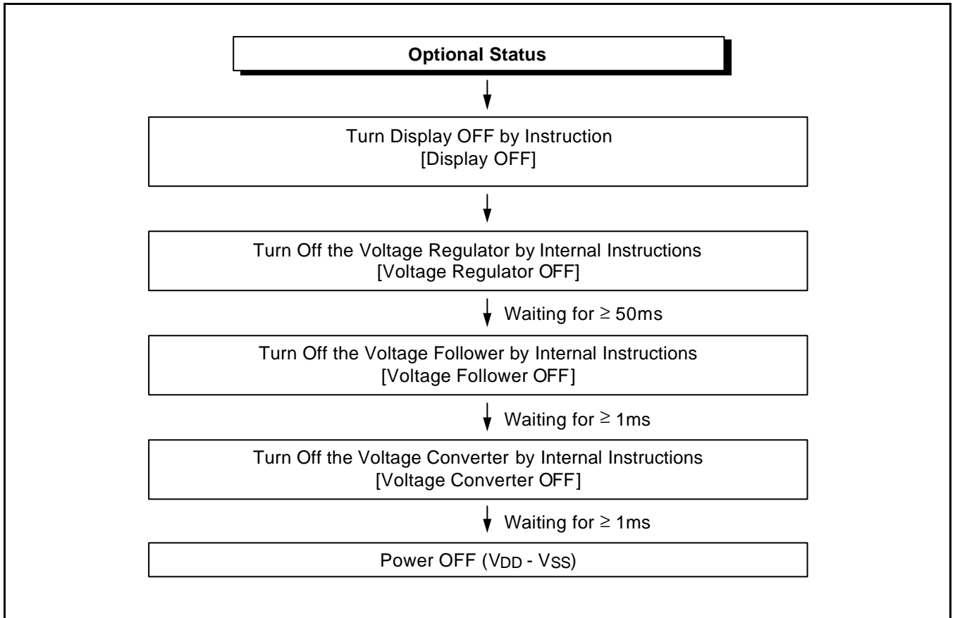
Figure 23. Power OFF
