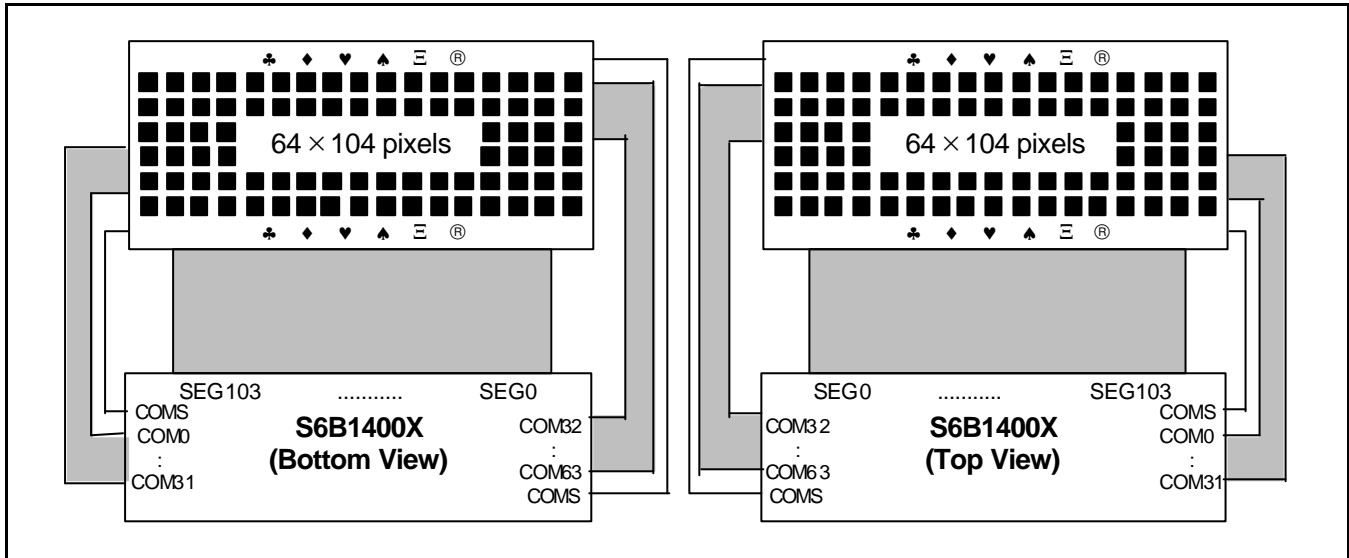
Figure 33. SHL = 1, ADC = 1
