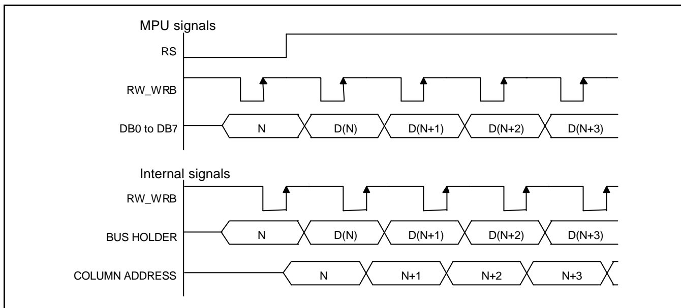
Figure 5. Write Timing
