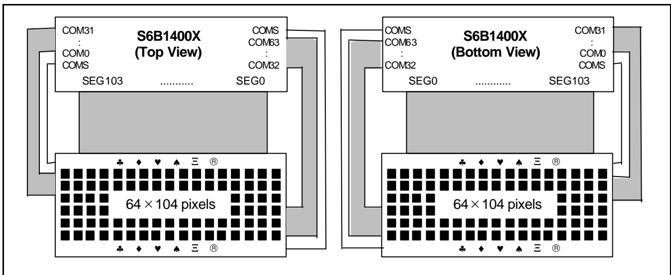
Figure 35. SHL = 0, ADC = 1
