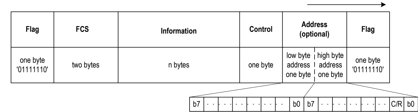
Figure 12. Standard HDLC Packet
