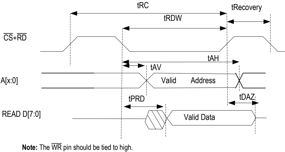
Figure 49. Intel Non-Multiplexed Mode Read Cycle
