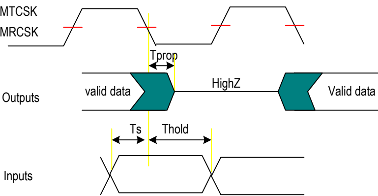
Figure 42. I/O Timing in Multiplexed Mode
