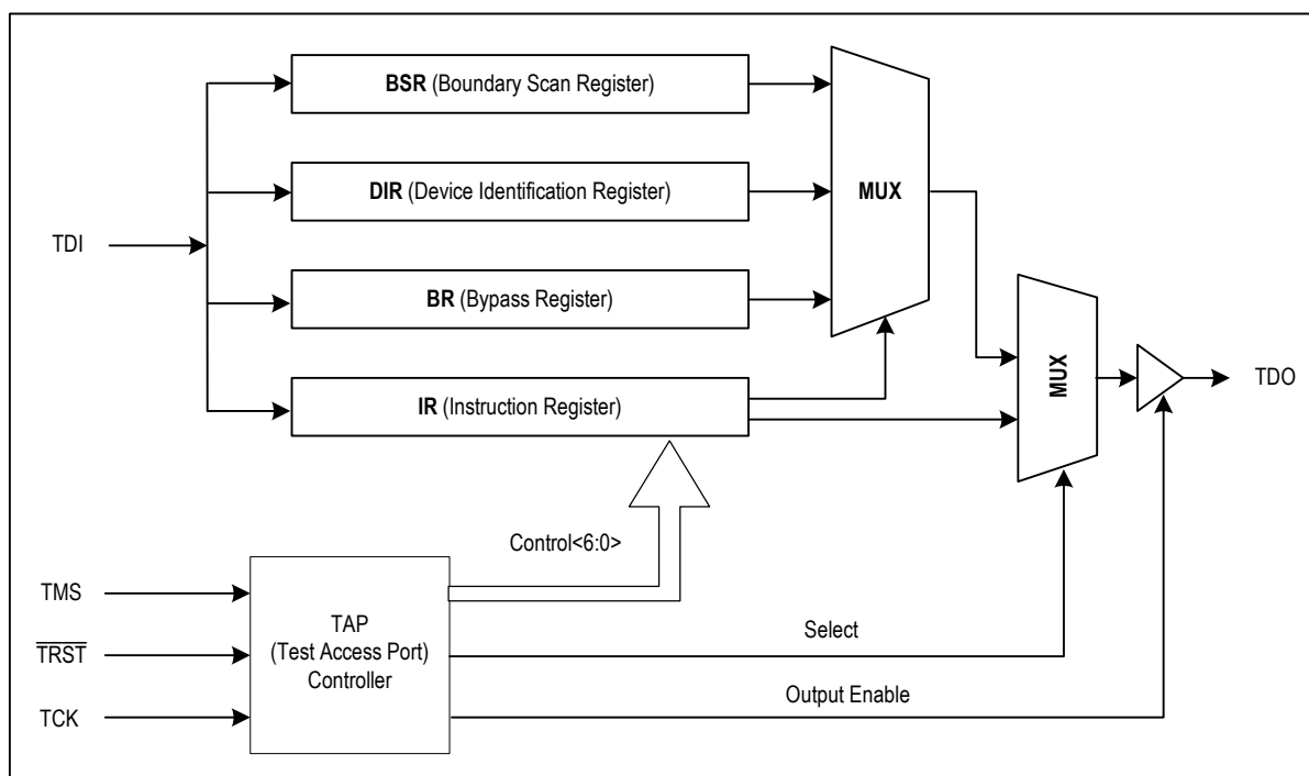
Figure 39. JTAG Architecture
