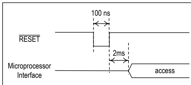
Figure 36. Hardware Reset In Normal Operation
