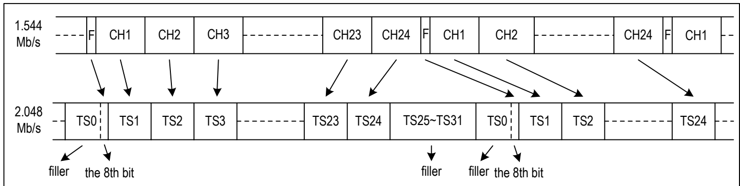
Figure 19. T1/J1 To E1 Format Mapping - Continuous Channels Mode
