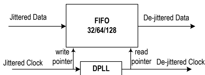
Figure 5. Jitter Attenuator
