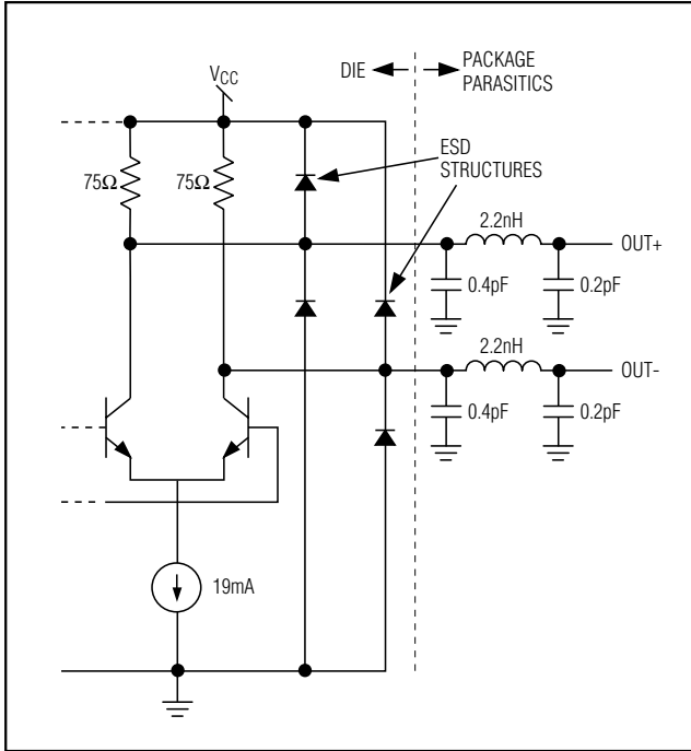
Figure 4. MAX3752/MAX3753 Output Structure
