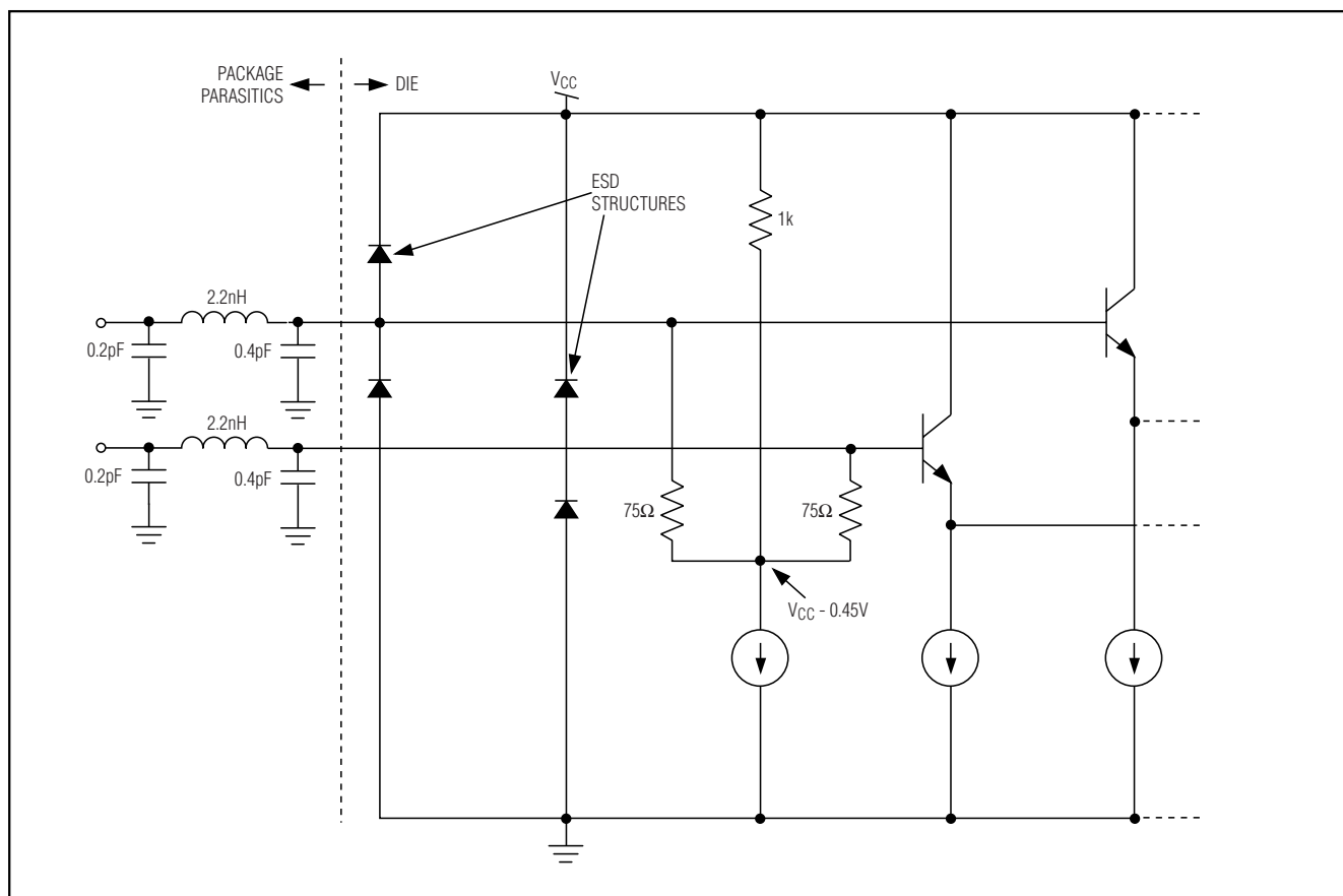
Figure 3. MAX3752/MAX3753 Input Structure
