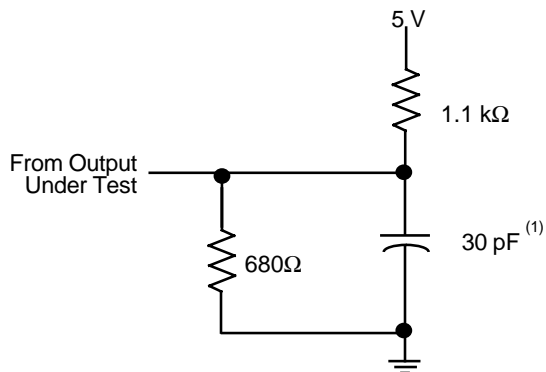
LOAD CIRCUIT
