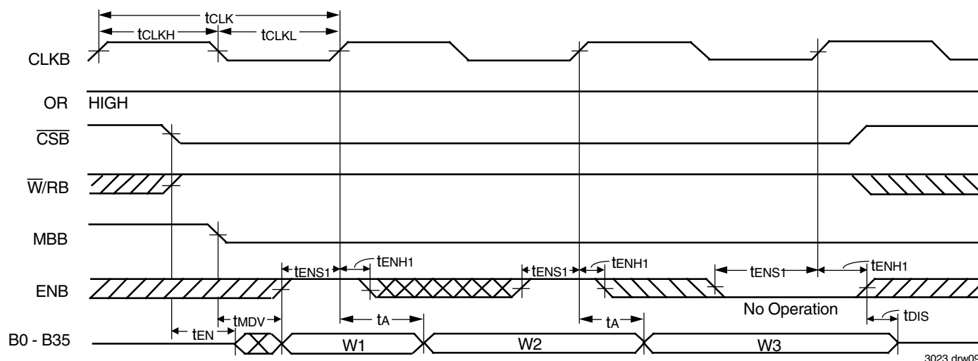
Figure 6. FIFO Read Cycle Timing
