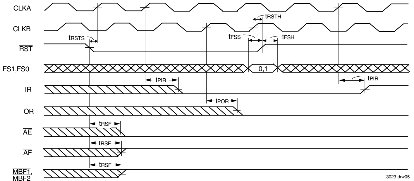
Figure 2. FIFO Reset Loading X and Y with a Preset Value of Eight
