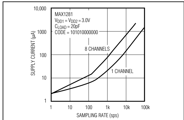
Figure 10b. Average Supply Current vs. Sampling Rate (Using FULLPD and External Reference)
